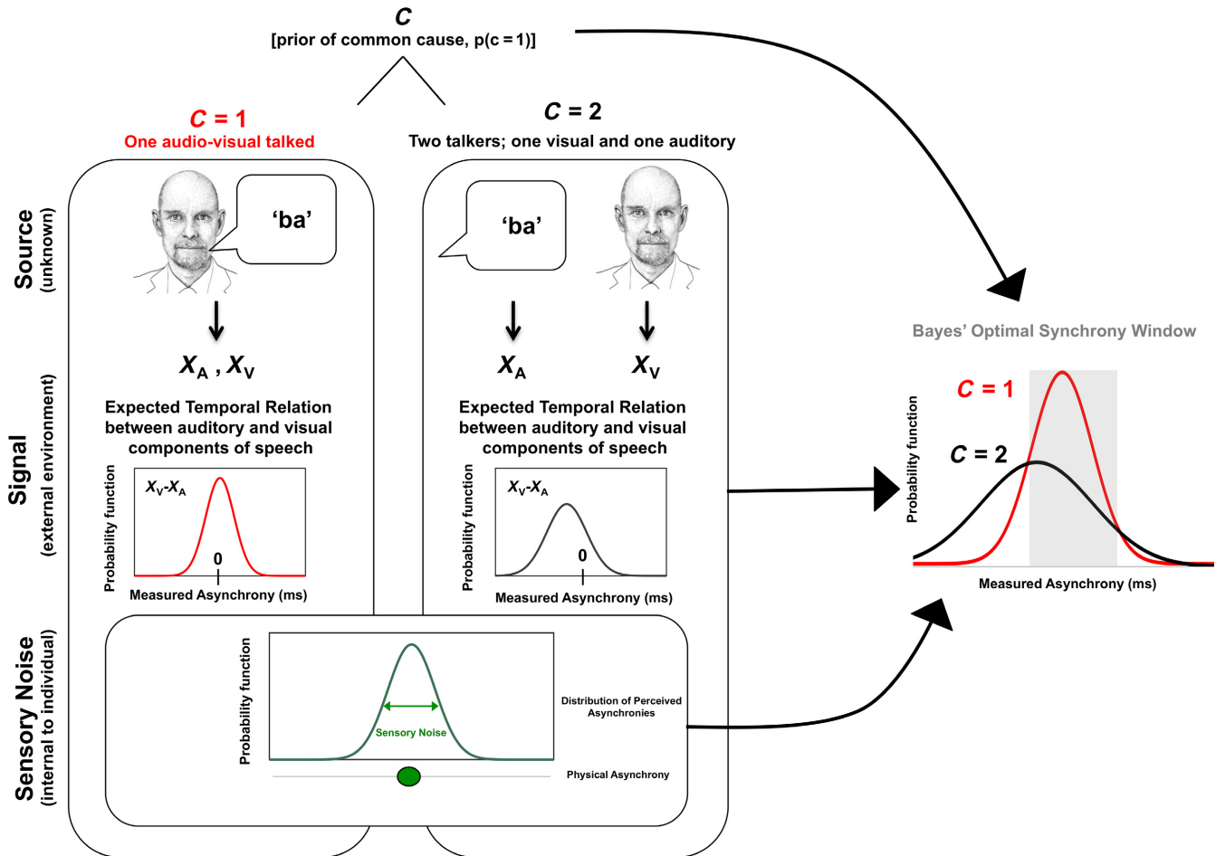
FIG. 1. Causal inference model of audiovisual speech. Participants possess a prior tendency to bind sensory information together across time ( P(C = 1) , at the top) and sample the sensory world with a certain degree of noisiness ( \sigma_{\text{sensory noise}} , at the bottom). When auditory and visual stimuli are taken to emanate from the same cause, the likelihood distribution where these signals stem from in the world has a relatively narrow variance ( \sigma_{C=1} ) and a mean ( \mu_{C=1} ) equal to zero. In contrast, when these signals emanate from different causes, the likelihood from which they stem has a relatively large variance ( \sigma_{C=2} ), as they are independent from one another, and a negative mean ( \mu_{C=2} ) in comparison with \mu_{C=1} . These parameters are all related via Bayes' rule (Eqn 2) and define the Bayes' optimal synchrony window (right).
