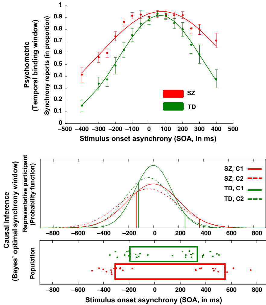
FIG. 4. Temporal binding window and Bayes' optimal window of synchrony judgments for SZ and TD participants. Top panel: averaged proportion of synchronous responses ( y -axis) as a function of stimuli onset asynchrony (SOA, negative values indicate audio-leading SOAs and positive values indicate visual-leading conditions) and fit to the average (for visualization only). Temporal binding windows—indexed via Gaussian fitting—for audiovisual speech stimuli are larger for SZ (red) than TD (green) participants. Error bars represent \pm 1 SEM. Bottom panel: Top, C = 1 (continuous) and C = 2 (dashed) distributions as a function of SOA for a representative SZ (red) and TD (green) participant. Bottom panel: population data for SZ (red) and TD (green) participants. Each participant is represented by two dots, one at position x < 0 and one at position x > 0 along the x -axis. The median for each group is represented via a box, the length of which illustrates the Bayes' optimal window of synchrony judgment for each group.
